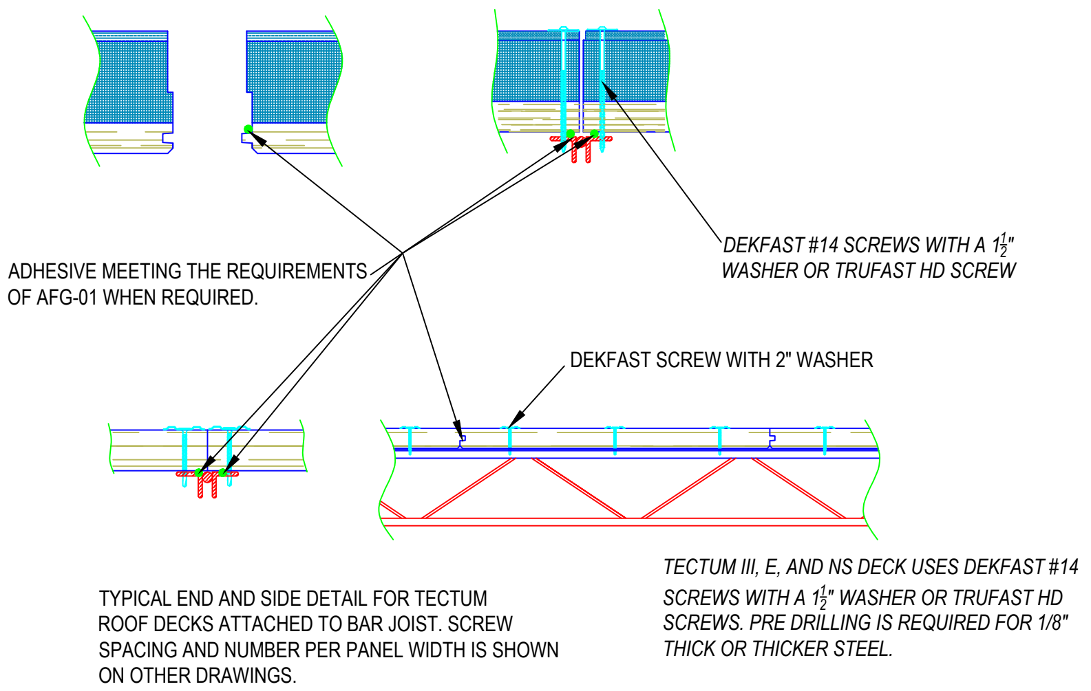
1 DECK SCREWED TO BAR JOIST Scale: N.T.S.
